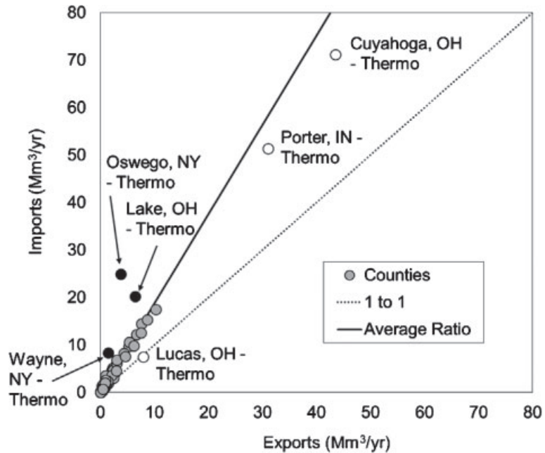
Figure 7. Virtual stream depletion exports and imports for the US portion of the Great Lakes basin by county.
